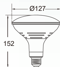
Base Type :E27
